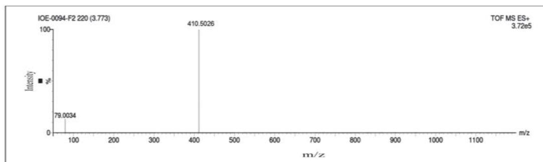
Fig. No. 1: LCMS spectra of Leaf extract (Ethanol) of R. nasutus
