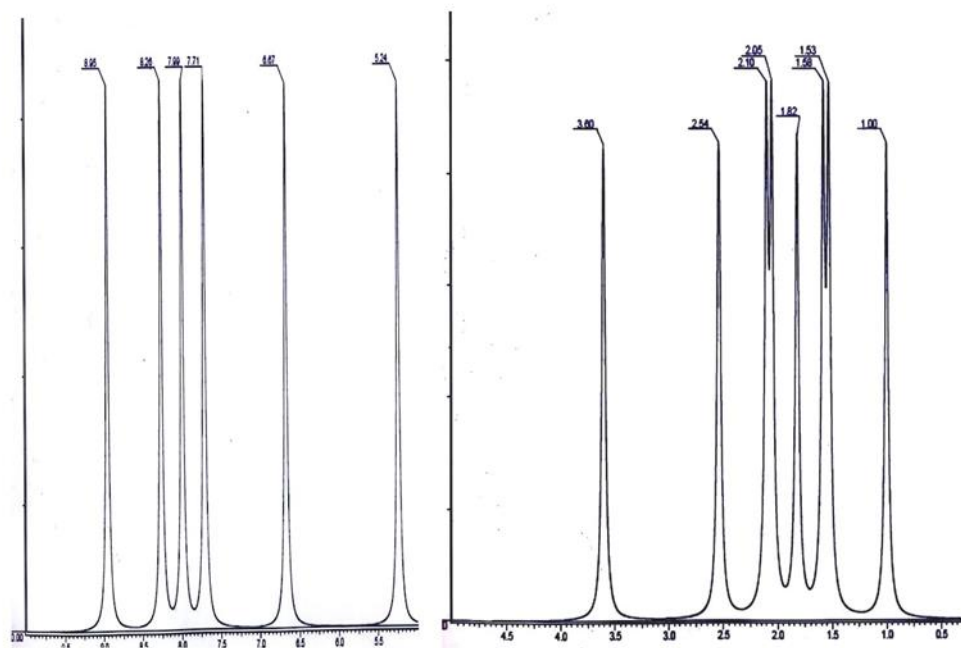
Fig. No.2: NMR (H) spectra of Leaf extract (Ethanollic) of R. nasutus
