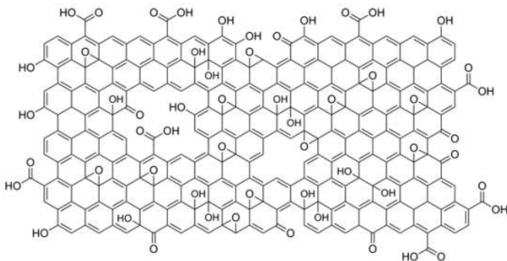
Figure 2: Graphene oxide model (GO)
